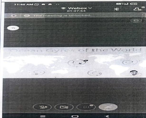
OCEAN GYRES OF THE WORLD
